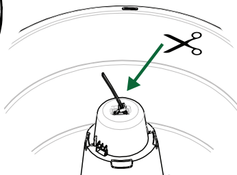
Zip Tie spec: width: 4.8mm length: min. 600mm
